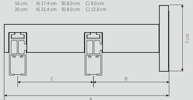
16 cm / 20 cm double wall bracket rectangular
